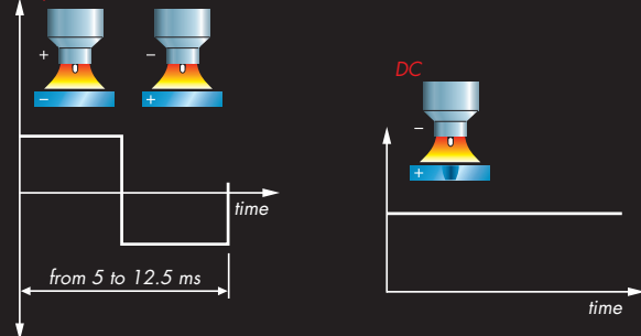
Square wave AC
